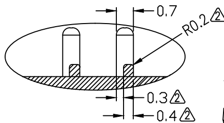
SEC. B-B SCALE 2 : 1 C
