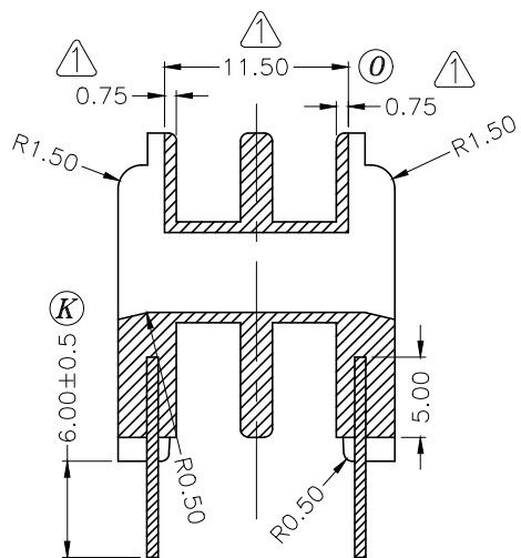
SEC B-B
