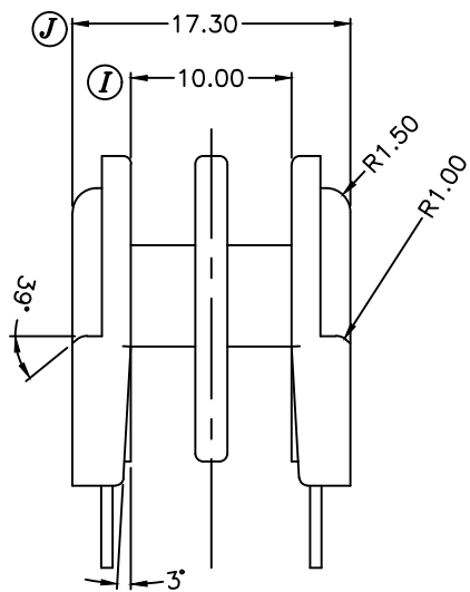
SEC B-B
