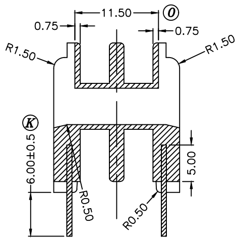
SEC B-B
