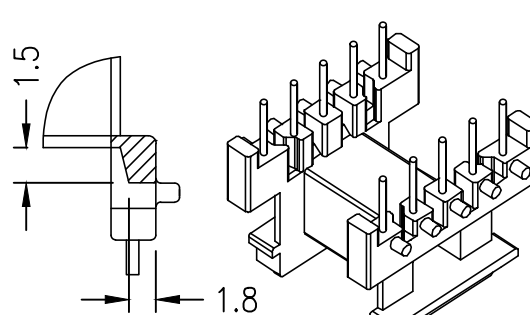
SECTION A-A FOR THE SLOTS BETWEEN PINS 1-2, 4-5, 6-7, AND 9-10.
