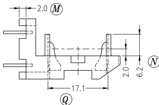
PART P-2401
