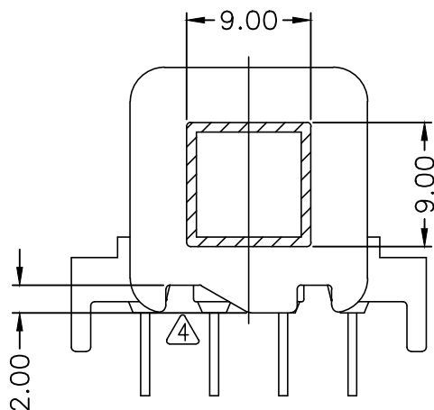
SEC B-B
