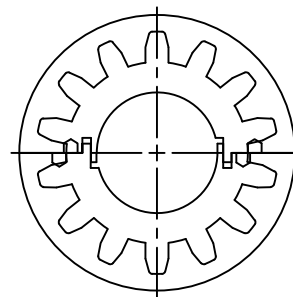
PART P-3501
