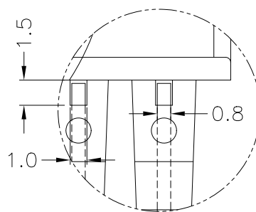
DETAILS A SCALE 3:1
