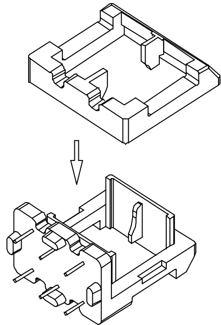
PART P-3502
