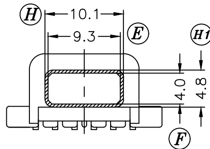
SECTION B-B
