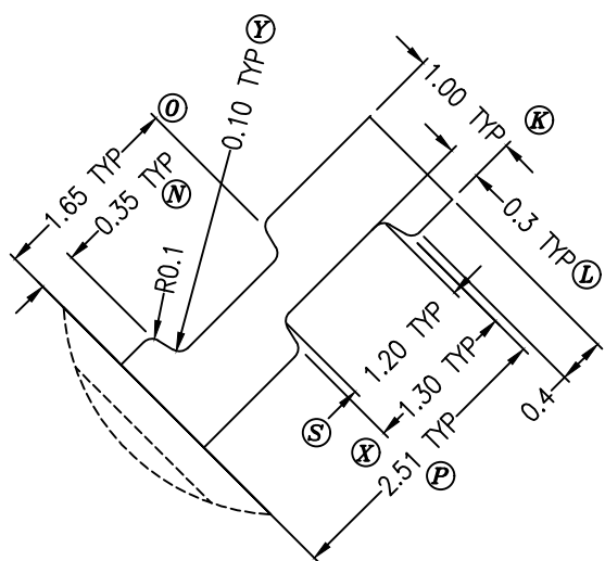
DETAIL A SCALE 3:1
